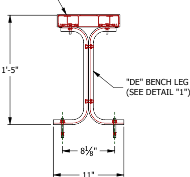
CONCRETE ANCHORED OPTION SEE DETAIL "3"
